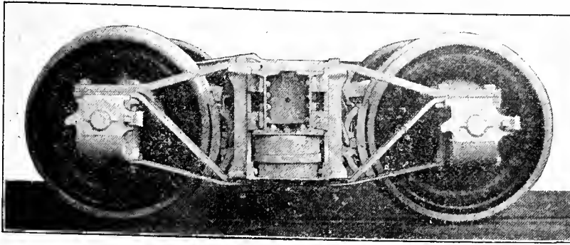
Fig. 4576. Side View. FREIGHT-CAR TRUCK. HARVEY STEEL CAR & REPAIR WORKS.
